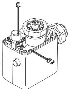
Valve Body Assembly* (* may vary in appearance depending on model. TET1UBi*#CP model shown.)
